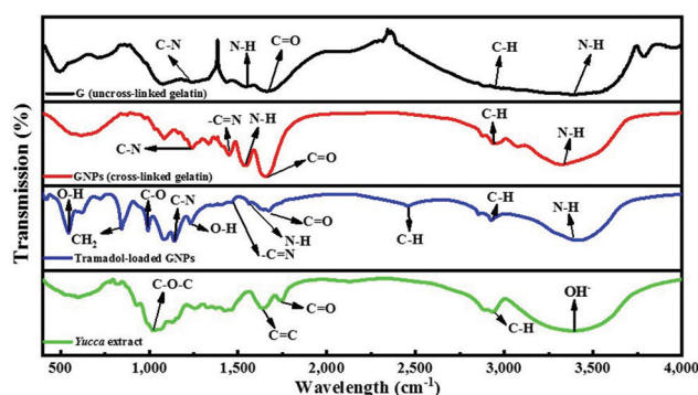
Figure 2. The Fourier transform infrared spectroscopy spectra of gelatin (G; uncross-linked gelatin), GNPs; cross-linked gelatin, tramadol-loaded GNPs, and Yucca extract. Abbreviation: GNPs: Gelatin nanoparticles.
