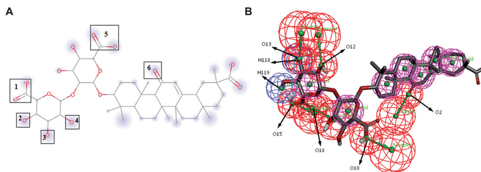
Figure 6. A pharmacophore model of glycyrrhizin, highlighting functional groups involved in the interaction with the 6VXX target protein. (A) Pharmacophore moieties are marked with numbers: 1, 5 as carboxyl groups ( \text{COOH} ); 2, 3, and 4 as hydroxyl radicals ( \text{OH} ), and 6 as a ketone group ( =\text{O} ). (B) A pharmacophore model of glycyrrhizin showing H-acceptors in red, H-donors in blue, hydrophobic groups in violet, and their centers are indicated by labels and symbols
