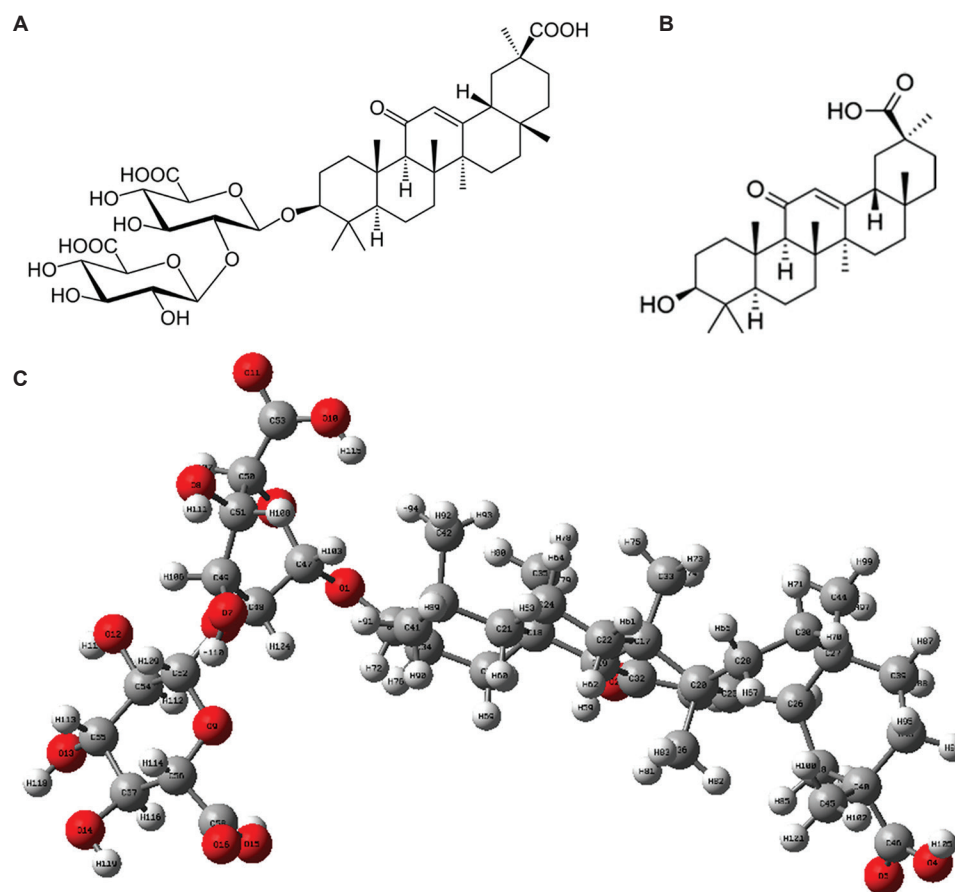
Figure 1. Chemical structure of (A) glycyrrhizin and its part (B) glycyrrhetic acid, showing the atoms of the molecule in the order in which they are bonded. Molecular structure with (C) atomic numbering scheme for glycyrrhizin, showing the spatial arrangement of atoms within this molecule using a ball-and-stick model
