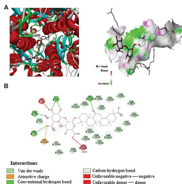
Figure 3. The molecular docking results of glycyrrhizin with 6VXX. (A) Three-dimensional visualization and (B) two-dimensional diagram of the receptor–ligand interactions. The ligand and receptor are depicted, and important interactions, including hydrogen bonds, attractive charge interactions, and others, are highlighted
