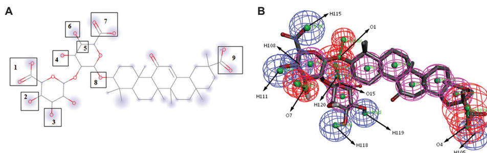
Figure 5. A pharmacophore model of glycyrrhizin, highlighting functional groups involved in the interaction with the 7ZQV target protein. (A) Pharmacophore moieties are marked with numbers: 1, 7, 9 for carboxyl groups ( -\text{COOH} ), 2, 3, 4, and 6 for hydroxyl groups ( -\text{OH} ), 8 for the ether group ( -\text{O}- ), and 5 for the aromatic CH group. (B) A pharmacophore model of glycyrrhizin showing H-acceptors in red, H-donors in blue, hydrophobic groups in violet, and their centers are indicated by labels and symbols
