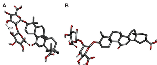
Figure 4. The optimal three-dimensional structure of glycyrrhizin corresponding to the best binding pose in the active site of the (A) severe acute respiratory syndrome coronavirus 2 (SARS-CoV-2) main protease (7ZQV) and (B) SARS-CoV-2 spike glycoprotein (6VXX), determined through molecular docking simulation
