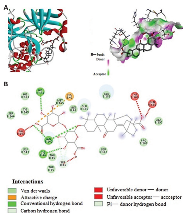
Figure 2. The molecular docking results of glycyrrhizin with 7ZQV. (A) Three-dimensional visualization and (B) two-dimensional diagram of the receptor–ligand interactions. The ligand and receptor are depicted, and important interactions, including hydrogen bonds, attractive charge interactions, and others, are highlighted
